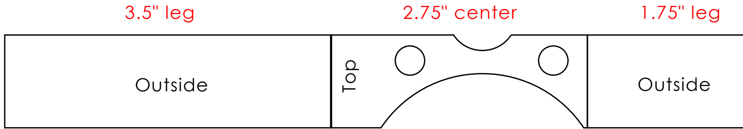
TOP PROFILE
